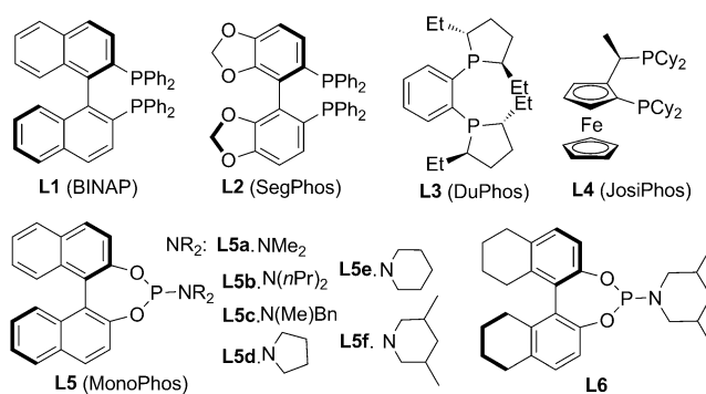
Figure 2. Structures of chiral ligands.
